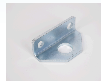
KP33000300Z 并柜吊环 Combination angle
