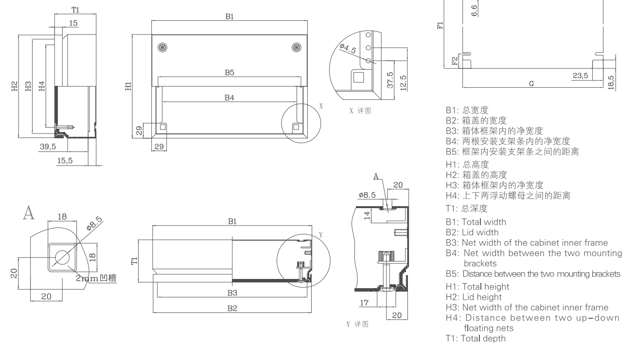
SKL/BKL series detail drawing
