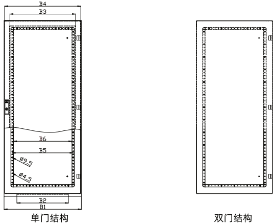
SAE/BAE series detail drawing
